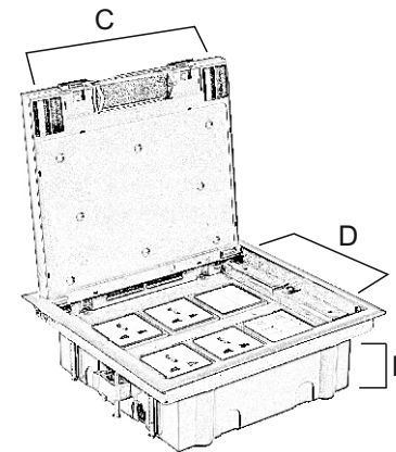
Cut-out Dimension
